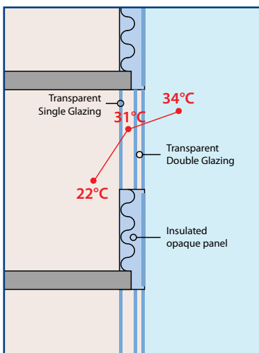
DOUBLE SKIN FACADE TEMPERATURE PROFILE IN SUMMER MODE
